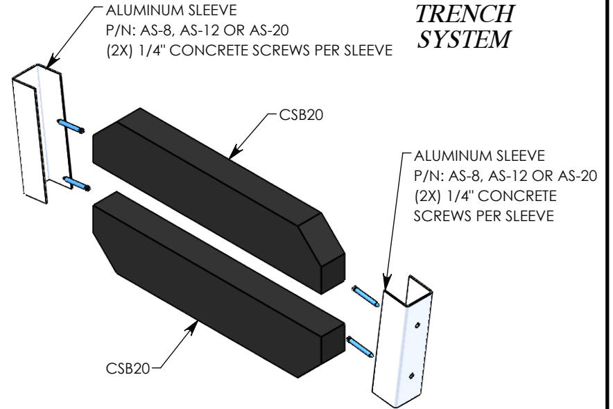
REFERENCE ASSEMBLY
