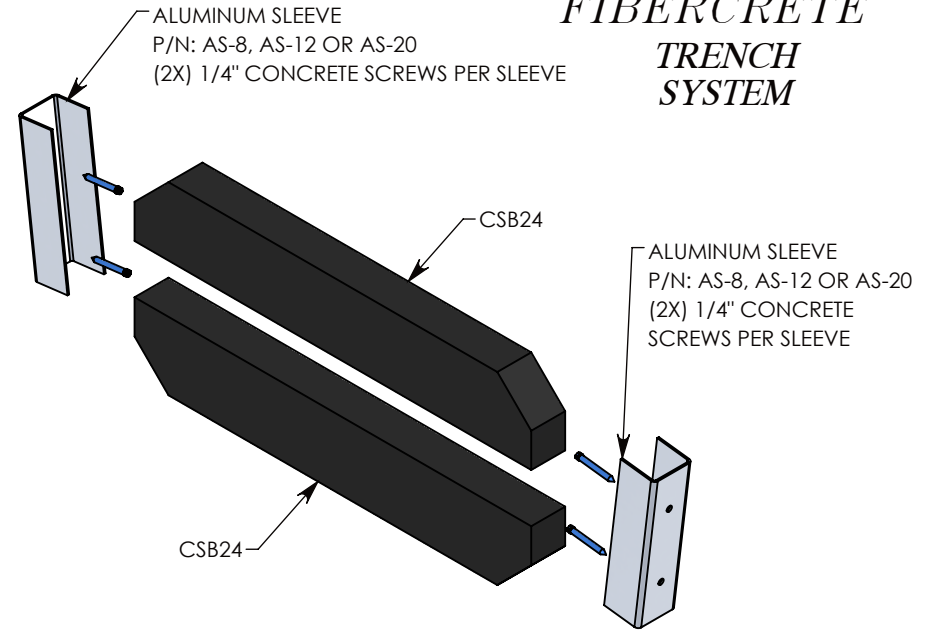
REFERENCE ASSEMBLY
