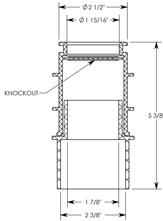
SECTION A-A SEAL RING HIDDEN
