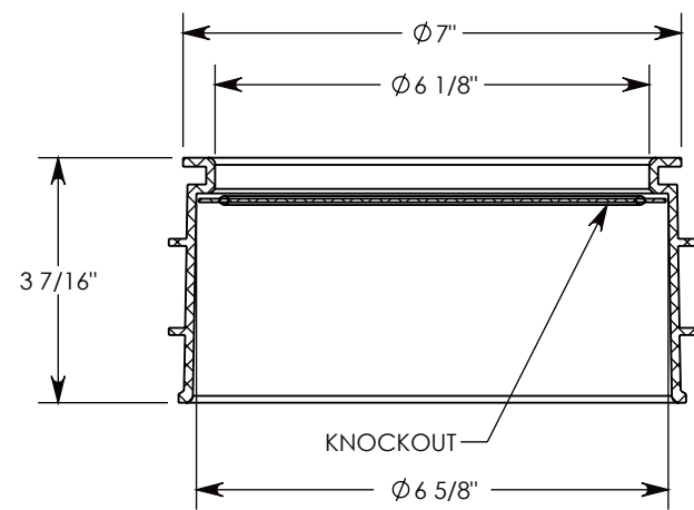
SECTION A-A SEAL RING HIDDEN
