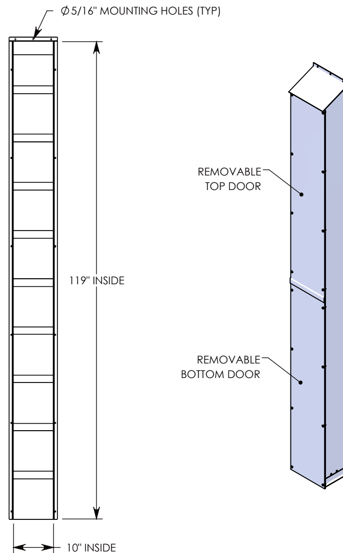
VIEW B-B
