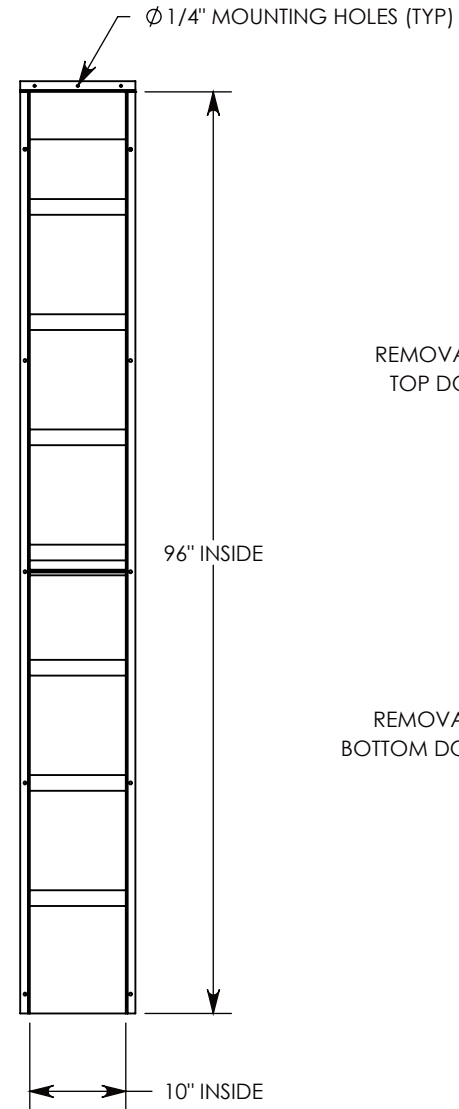
VIEW B-B
