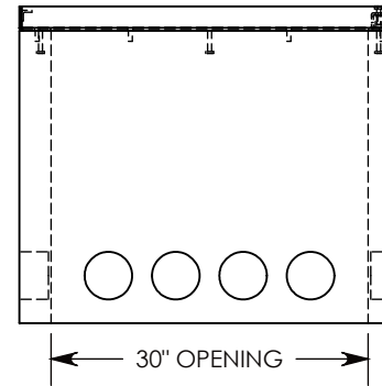
SIDE "C"
