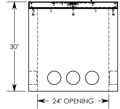
SIDE "D"
