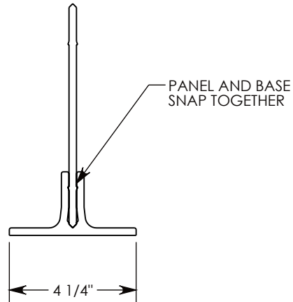
DETAIL A SCALE 2 : 9
